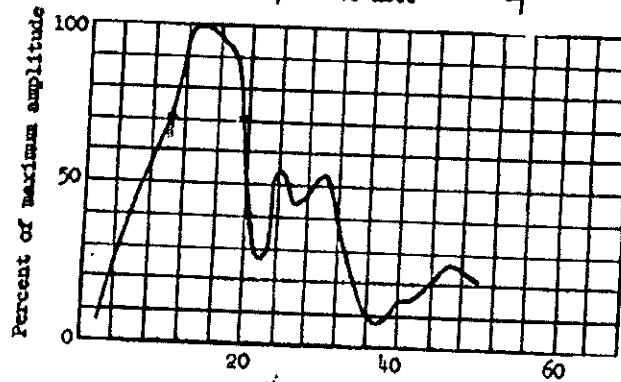
Fig. 3.80 Frequency function of broadband pulse Shot No. 7 1000 km from ground zero
